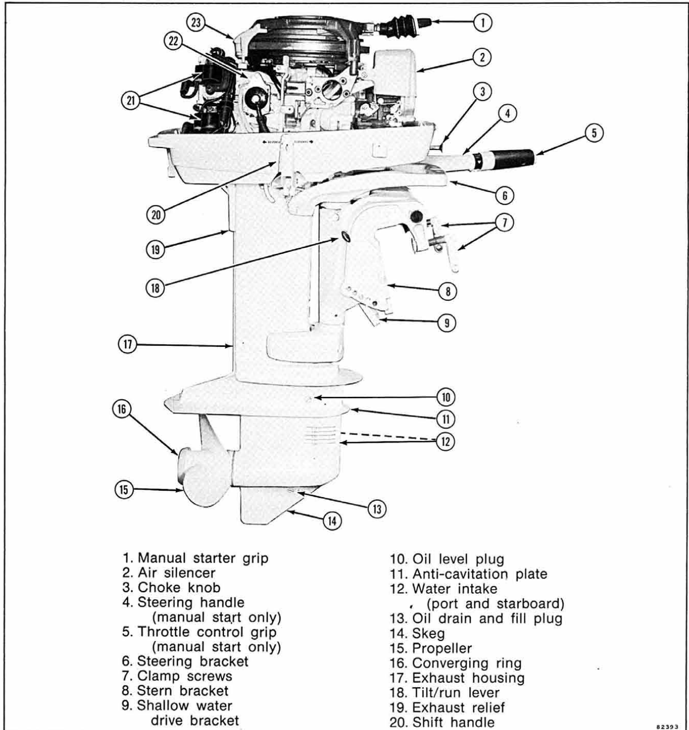
Figure 1-1. Starboard View - 35 HP Manual Start
