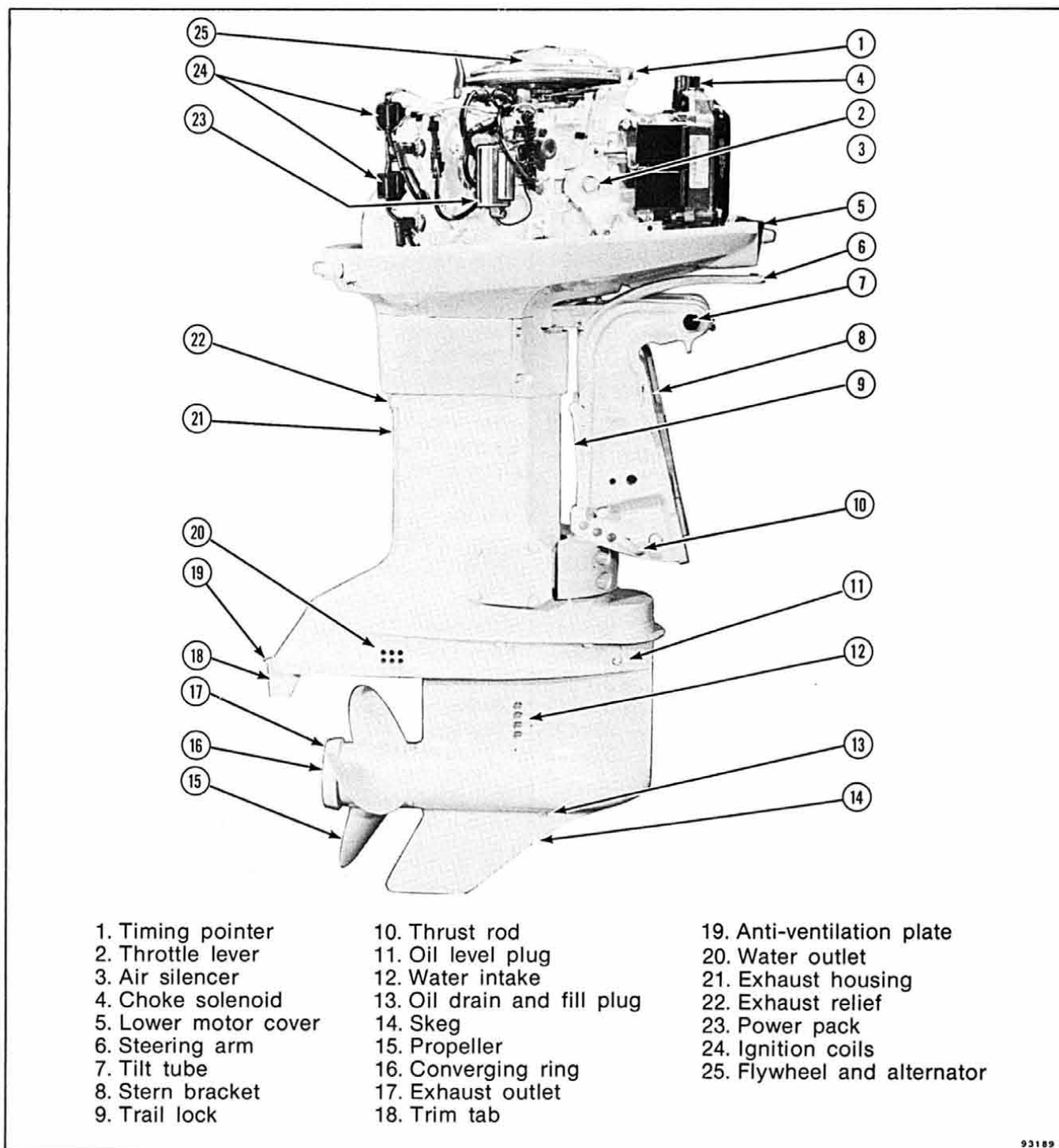
Figure 1-1. Starboard View - 140 HP
